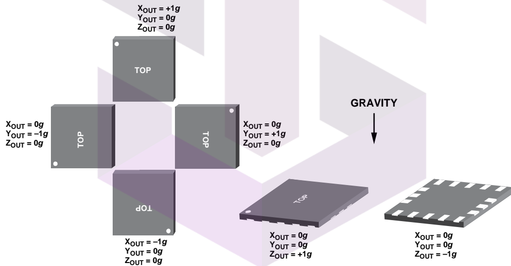
Figure 61. Output Response vs. Orientation to Gravity
