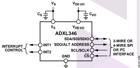
Figure 44. Applications Diagram
